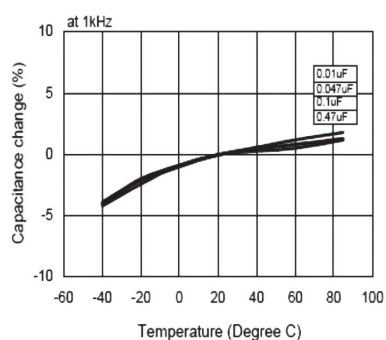
Temperature Characteristics
