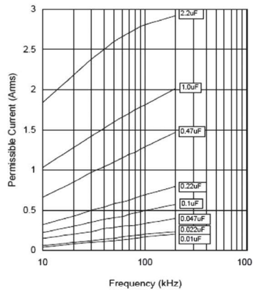
Permissible Current
