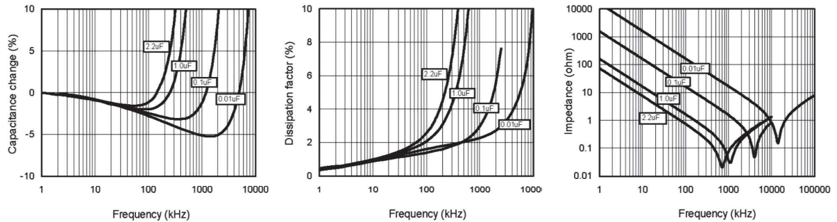
Frequency Characteristics
