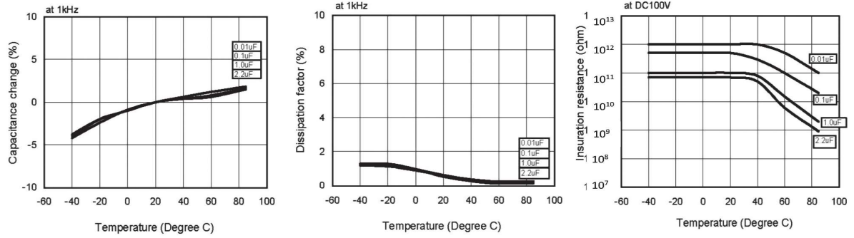
Temperature Characteristics
