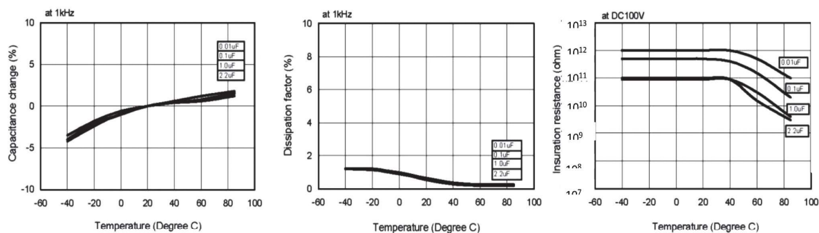
Temperature Characteristics
