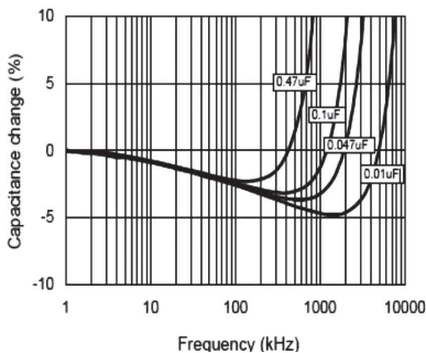
Frequency Characteristics
