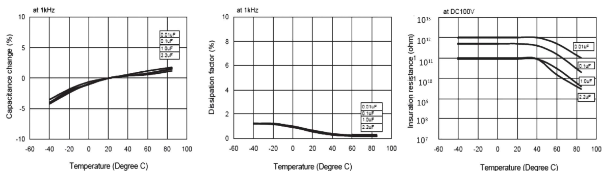
Temperature Characteristics
