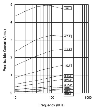
Permissible Current
